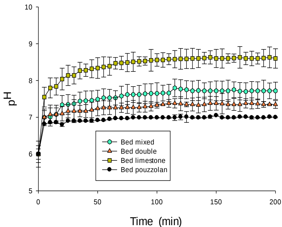
Figure 6: Variation of pH as a function of time in the configuration of filter beds on (H: 40cm; T: 23 \pm 2 °C; Turbidity: 30 \pm 1 , pH: 6 \pm 0.05 ; speed: 9.8 cm.min -1 )
