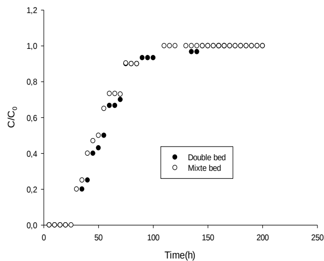
Figure 4: Breakthrough curve of the tracer (glucose) in the double and mixed bed pozzolan-limestone (H: 40 cm; T: 23 \text{ }^{\circ}\text{C} \pm 2 ; speed: 9.8 \text{ cm} \cdot \text{min}^{-1} , °Brix: 3 \pm 0.1 )
